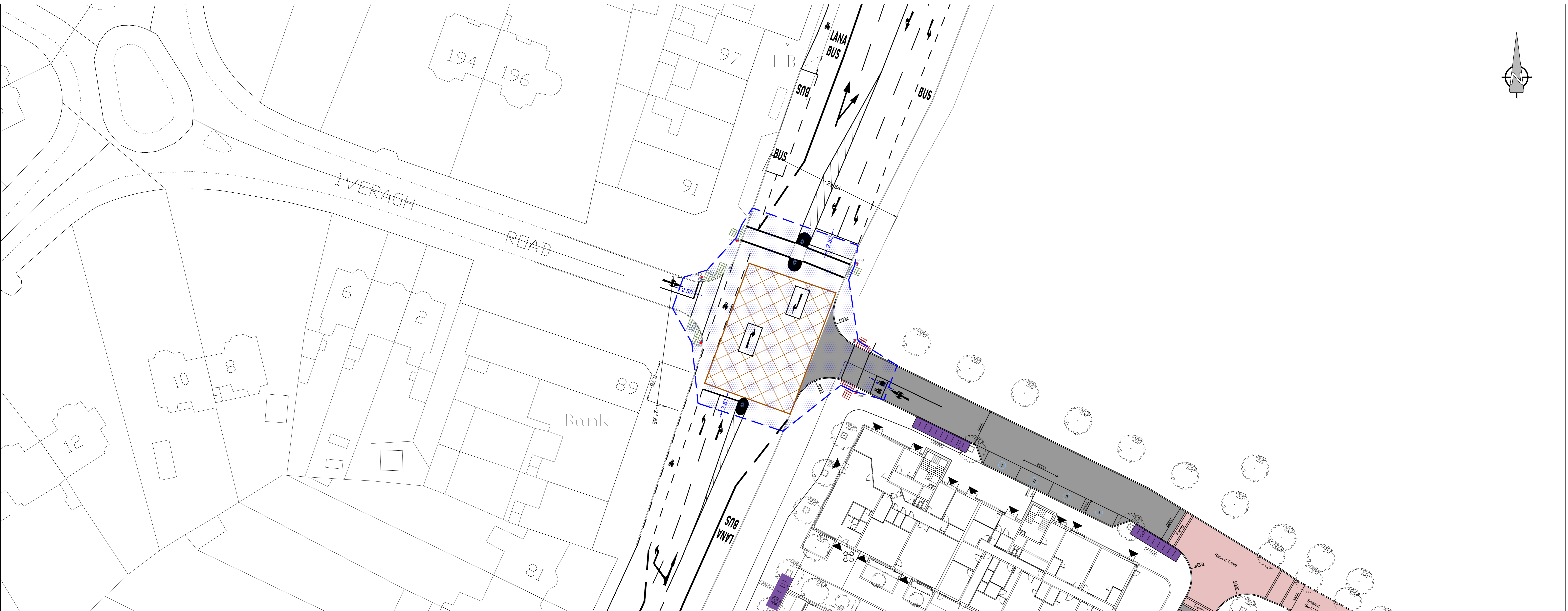
A JUNCTION VISIBILITY SPLAY Scale: 1:250 @ A0
